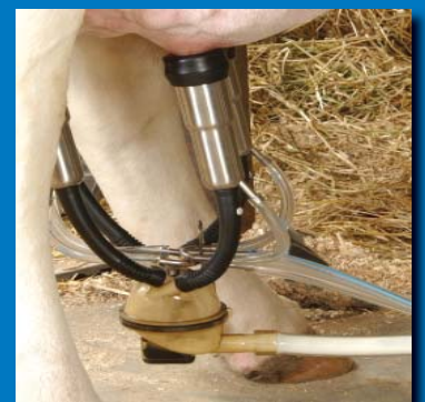
The MAX gives you top unloading action from a bottom unloading claw.
